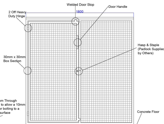
Front Elevation
